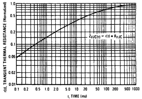
FIGURE 10 – THERMAL RESPONSE
